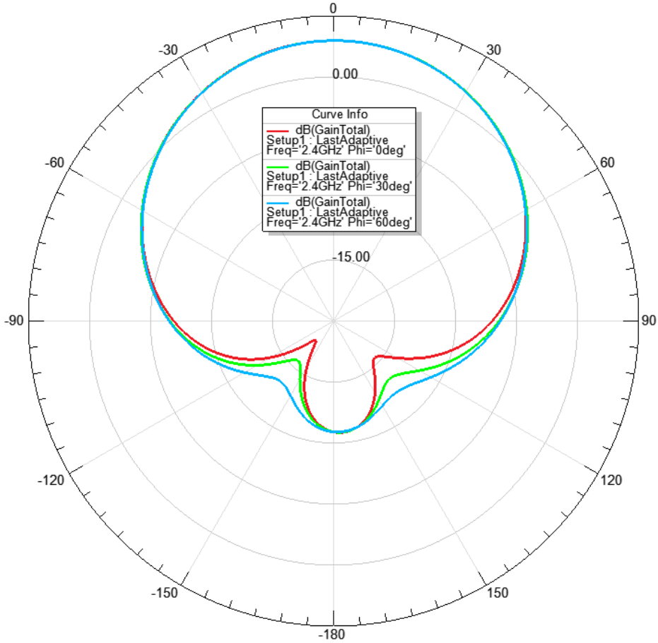
Gain Plot 13
